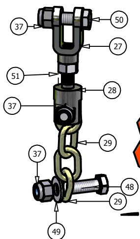
DETAIL E
