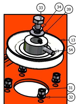
DETAIL C
