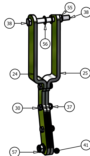
DETAIL C
